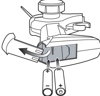
Transmitter
